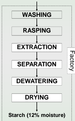
Figure 1: Unit operations of the cassava starch extraction process. The dotted line represents the selected system boundaries.
