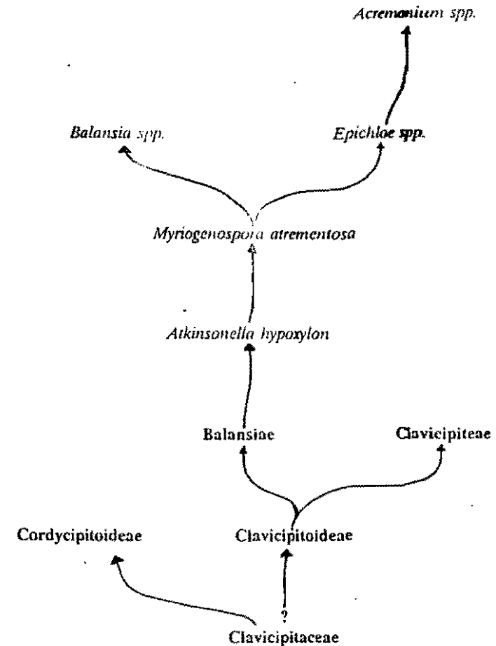
Figure 1. Possible evolutionary lines of taxa among grass endophytes of the tribe Balansiae within the family Clavicipitaceae, subfamily Clavicipitoideae, beginning with an unknown (?) ancestor. The tribe Clavicipiteae and the subfamily Cordycipitoideae are illustrated for possible relationships within the family, although no cladistics is implied.
