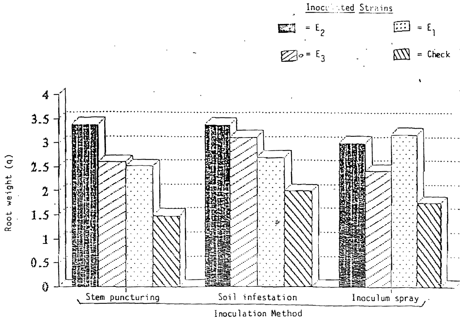
Figure 1.1. Effect of three endophyte species on root weight of one-month-old plants of three different clones (CG 1141-1, M Col 1418 and M Col 1505) inoculated by stem puncturing, soil infestation and inoculum spray with a mycelia suspension equivalent to 2 petri dishes/500 ml of distilled water.
