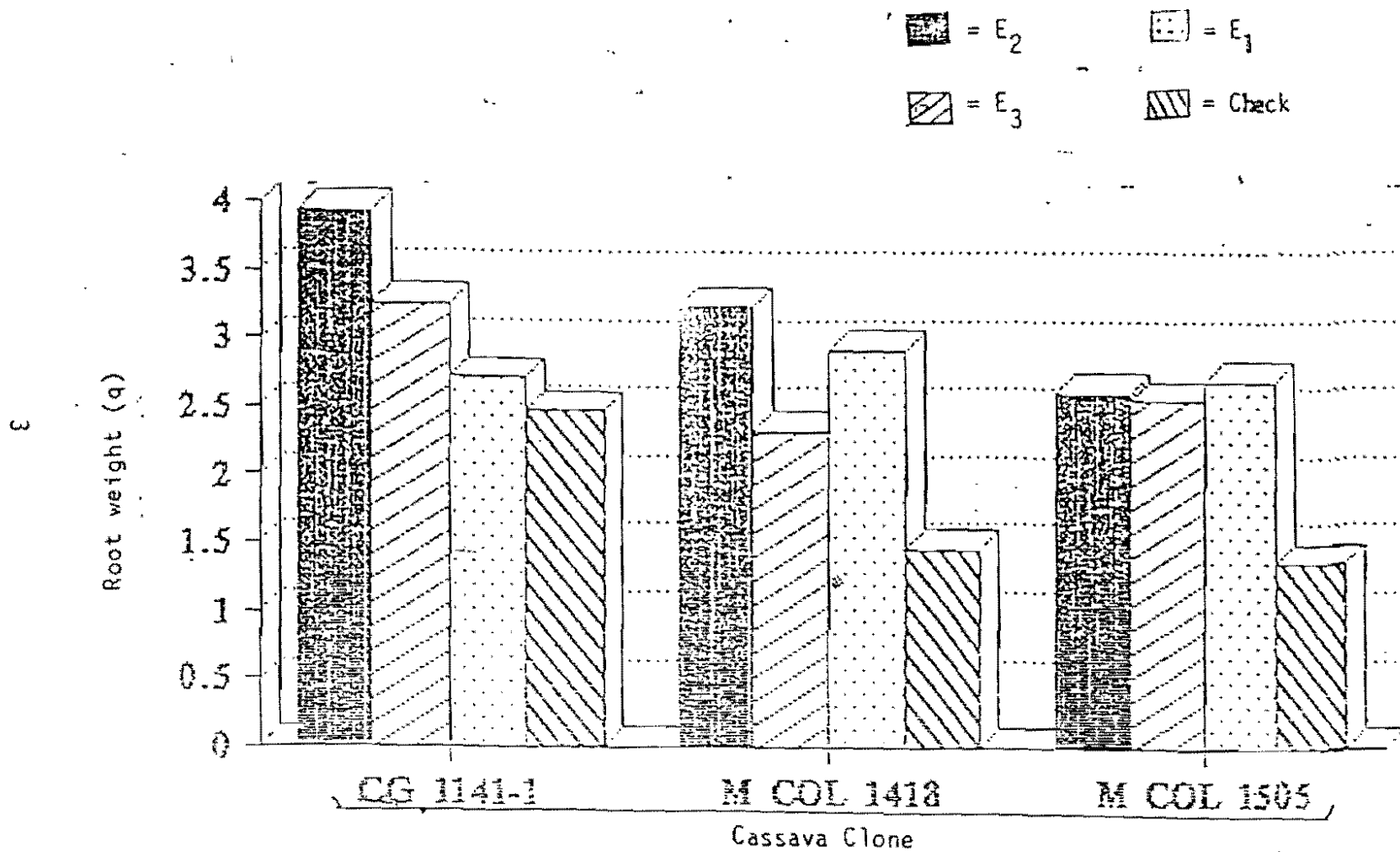
Figure 1.2. Effect of three endophyte species on root weight of plantlets of three cassava clones inoculated by three inoculation methods (stem puncturing, soil infestation and inoculum spray).
