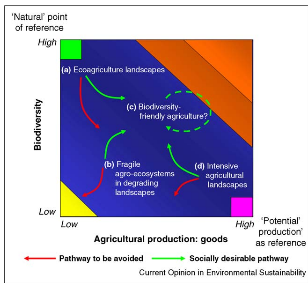
Possible tradeoffs between agricultural production and biodiversity. Modified after original drawing in [34].
