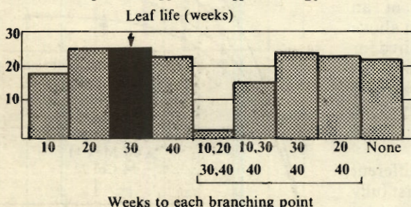
Figure 15. Simulated effects on yield of varying one character in a cassava plant with the following standards: branching at 30 weeks, leaf life of 10 weeks, population of 2 plants/m 2 , maximum leaf size of 500 cm 2 , and node weight of 1.0 gram. Arrows indicate standard type.
