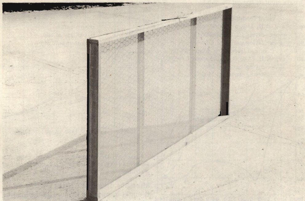
Figure 70. Drying trays constructed in this manner are sturdy and can carry 15 kg of moist chips m^2 .
