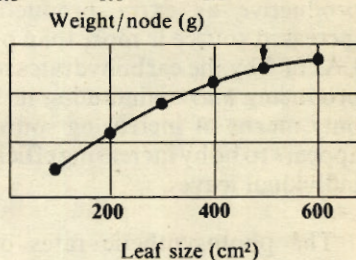
Figure 15. Simulated effects on yield of varying one character in a cassava plant with the following standards: branching at 30 weeks, leaf life of 10 weeks, population of 2 plants/m 2 , maximum leaf size of 500 cm 2 , and node weight of 1.0 gram. Arrows indicate standard type.
