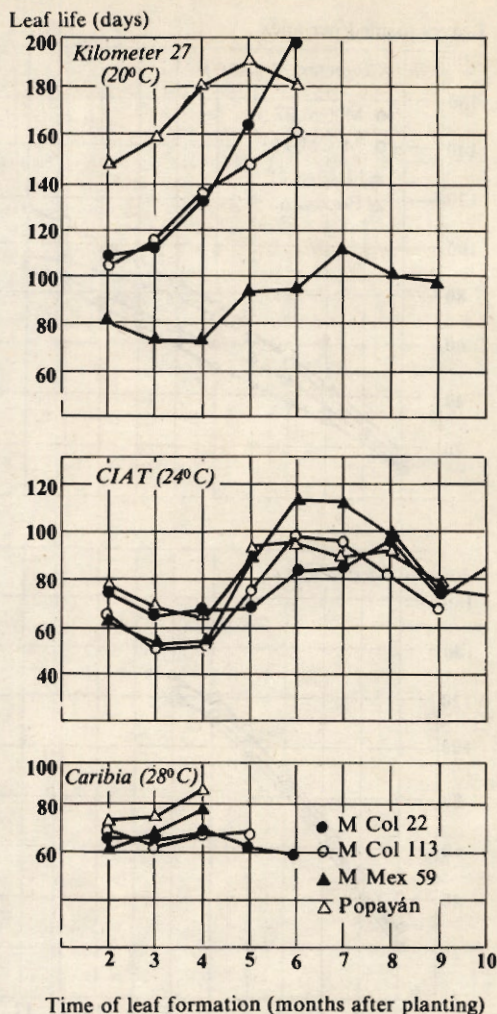
Figure 10. Leaf life of four varieties as a function of time after planting in three different temperature zones.
