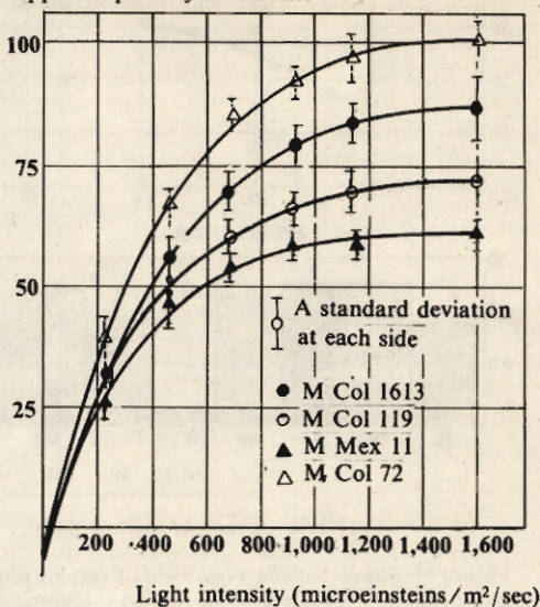
Figure 17. Photosynthetic rates of four different cassava clones.
