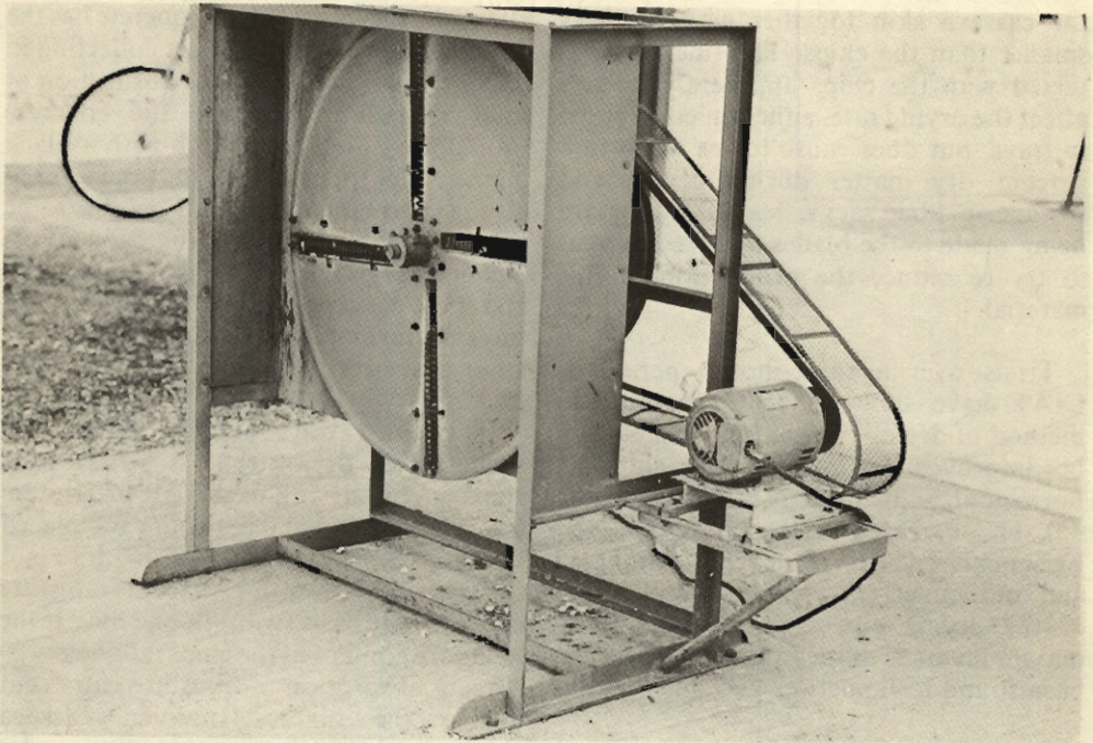
Figure 65. Malaysian type cassava chipper used in CIAT's studies of cassava drying.
