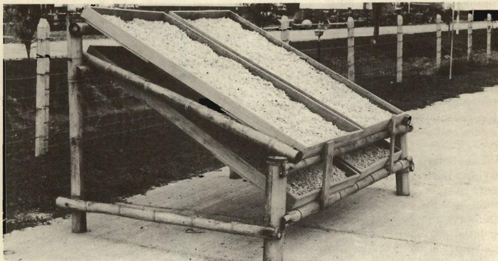
Figure 68. When inclined trays are stacked in this way with a 30-centimeter space between them, drying rates for the chips are not appreciably affected.
