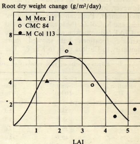
Figure 6. Changes in root dry weight as related to mean LAI 4-6 and 6-9 months after planting.
