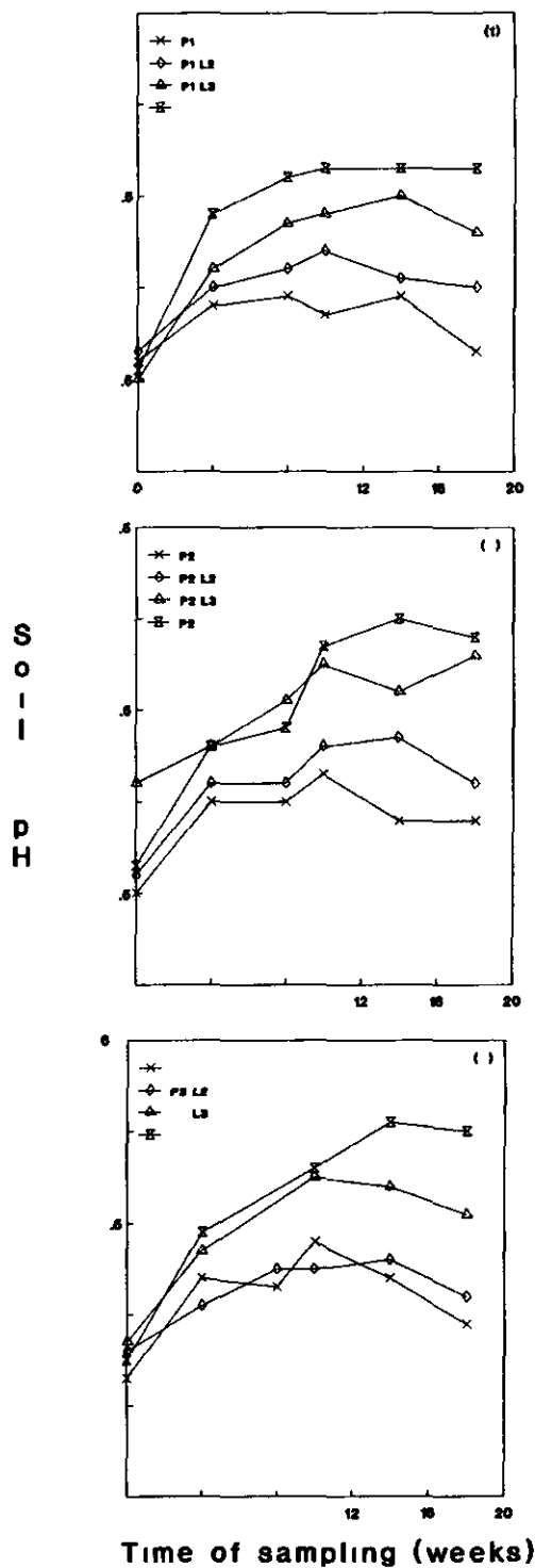
Figure 2 The effects of PR and lime on the soil pH
